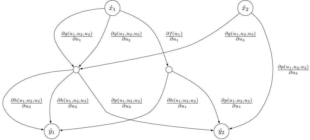
Figure 4: Linearization of the floating-point computation graph in Fig. 3. The inputs and outputs are the tangents associated with the corresponding primal values. Each edge is labeled with the partial derivative of its destination relative to its source, computed at the primal values in the associated primal floating-point computation graph. This graph can be interpreted as a structurally sparse representation of the Jacobian of the program in Fig. 2. It computes a Jacobian-vector product through forward mode by assuming scalar values flow through the network from input tangents to output tangents, interpreting an edge label as multiplication by a constant, and interpreting noninput vertices as summing their inputs. Note that conceptually, this approach could be extended to the case where variables hold vector values and primitive functions accept and return vector values by assuming vector values flow through the network, replacing the partial-derivative edge labels with partial Jacobians, interpreting the edge labels as matrix-vector multiplication, and interpreting noninput vertices as performing vector addition.
