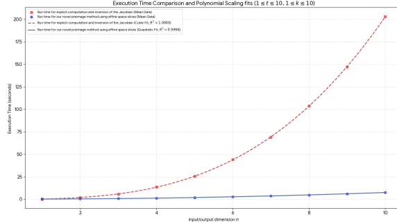
Figure 1: On-CPU Benchmark
